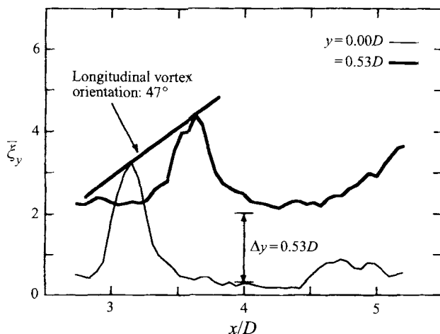
FIGURE 11. Distributions of transverse vorticity, \bar{\xi}_y(x) , in the streamwise direction at two y -positions across the wake, Re = 544 .
